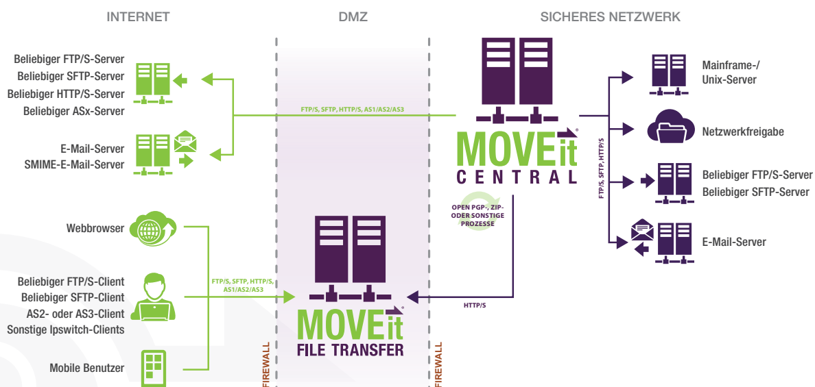
MOVEit Central Architecture
